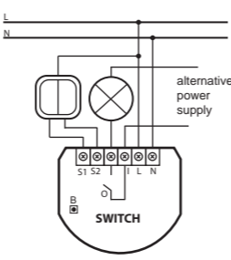
Fig.1 Wiring diagrams for Fibaro Switch.
